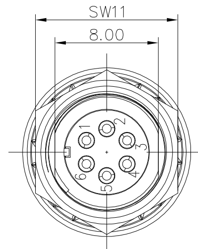
Soldering face
