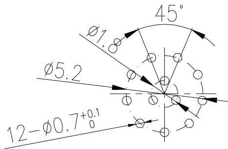
Recommended PCB size
