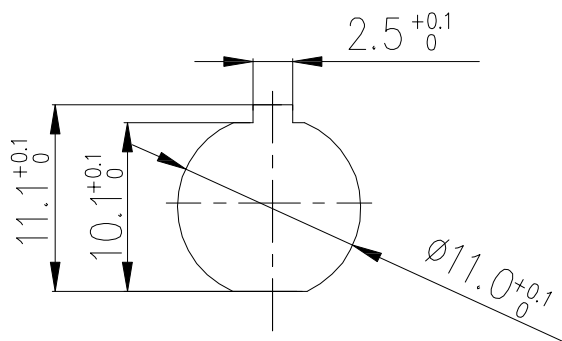
Recommended panel size
