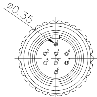
Mating Side
