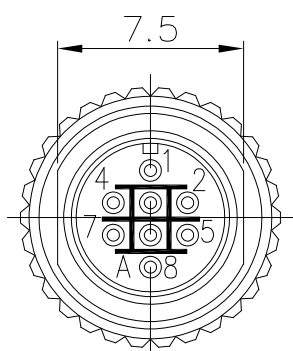
Solder Side
