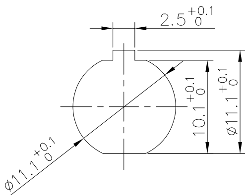
Panel dimensions
