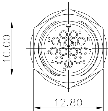
Soldering face
