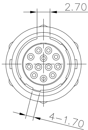
Mating face
