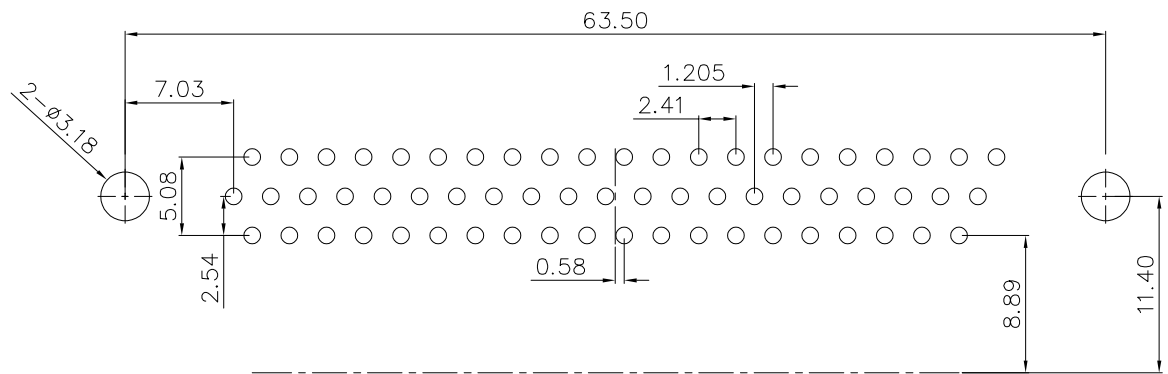
HD.D-SUB 62pin male right angle
