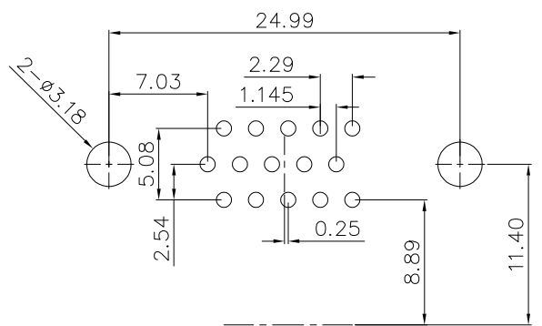
HD.D-SUB 15pin male right angle
