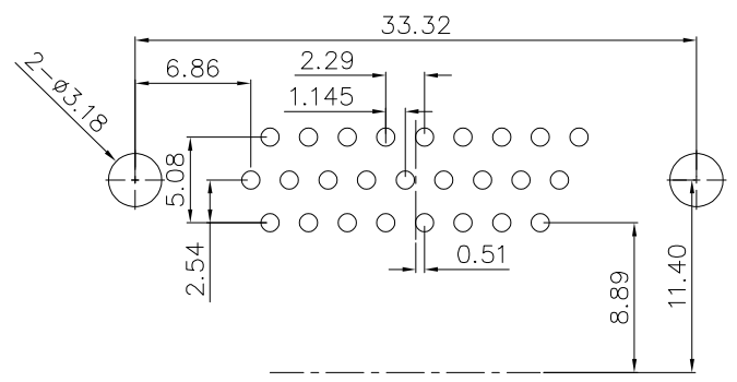
HD.D-SUB 26pin male right angle
