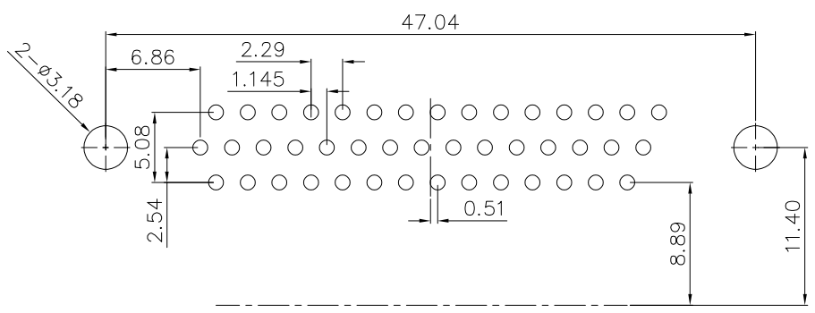
HD.D-SUB 44pin male right angle
