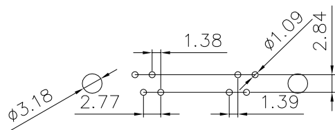
PCB layout
