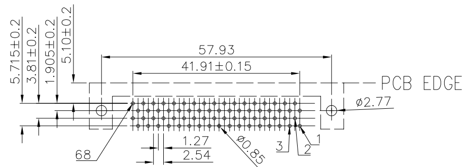
PCB layout
