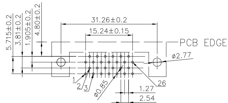
PCB layout
