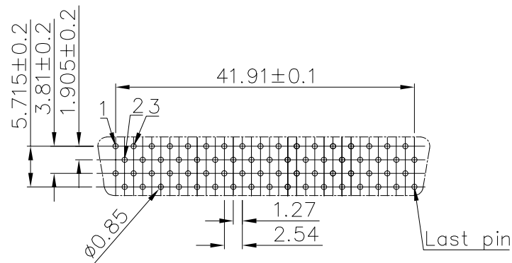
PCB layout A
