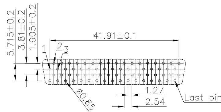
PCB layout B
