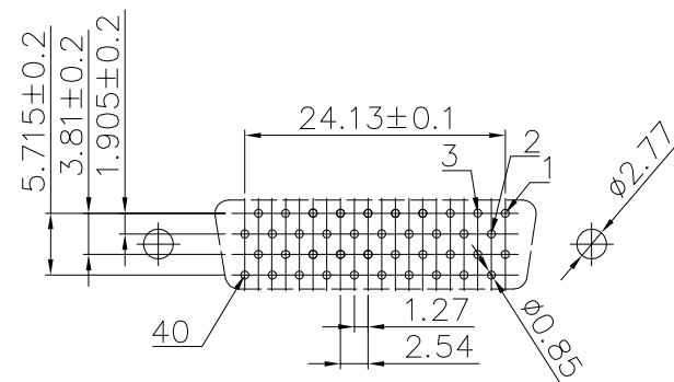
PCB layout
