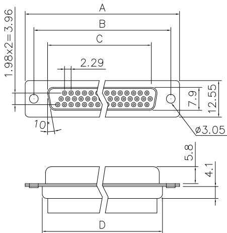
15,26,44,62pin
