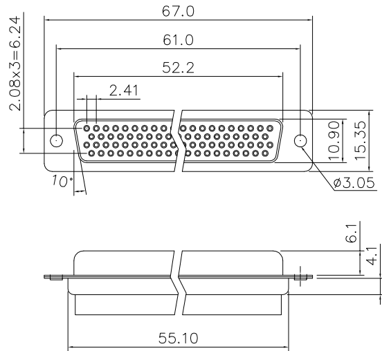
78pin
