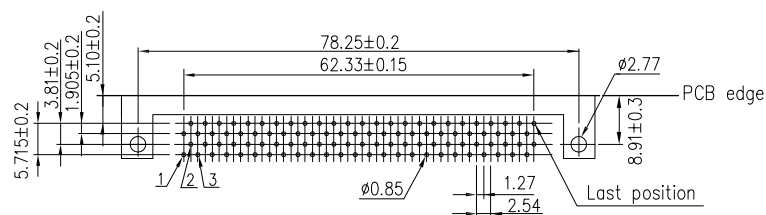
PCB layout
