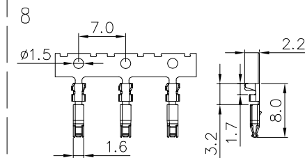
Brake terminal
