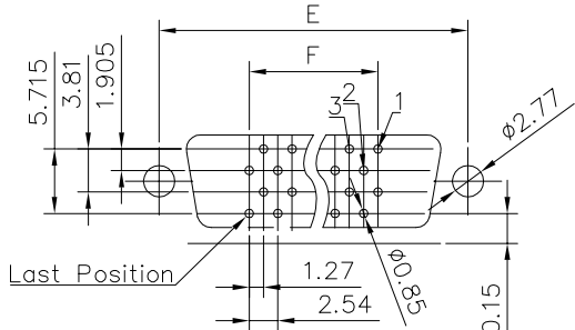
PCB Layout (20,36,40,68,100 Pos)
