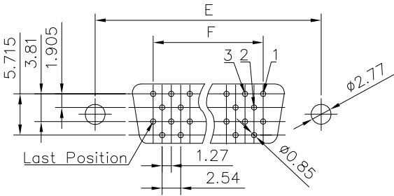
PCB Layout (14,26,50 Pos)
