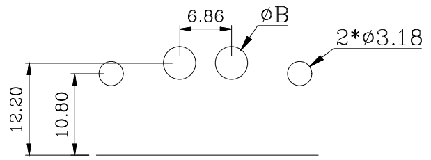
PCB LAYOUT
