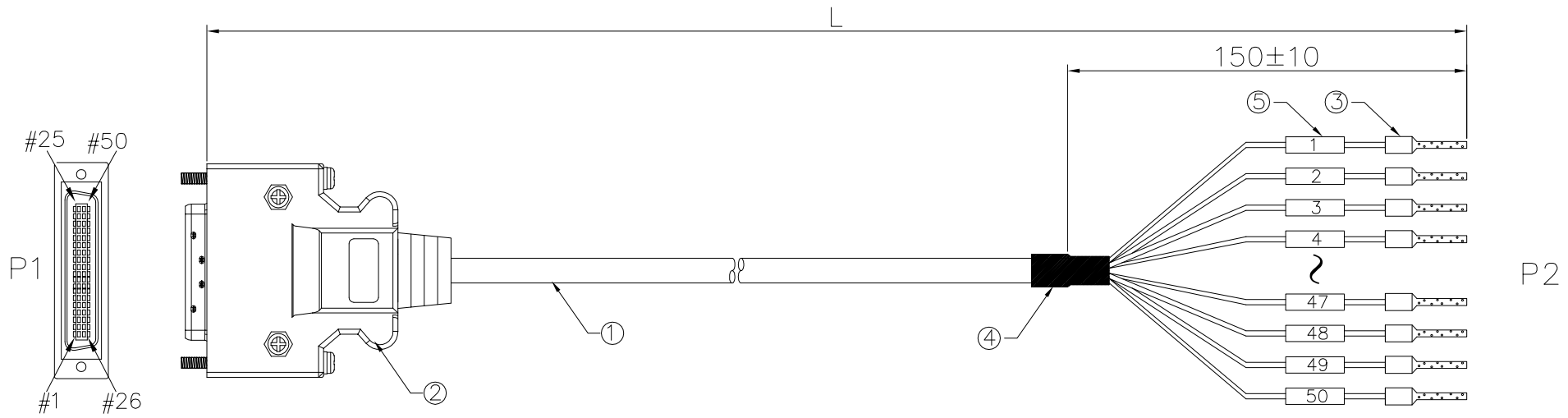
Pin assignment
