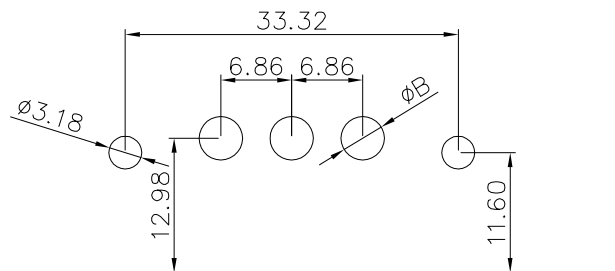
PCB layout
