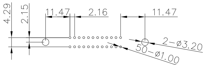
PCB layout
