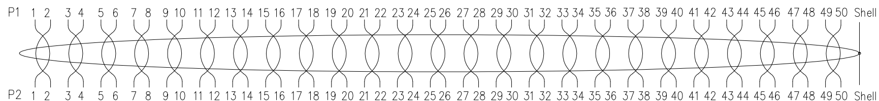
Pin assignment
