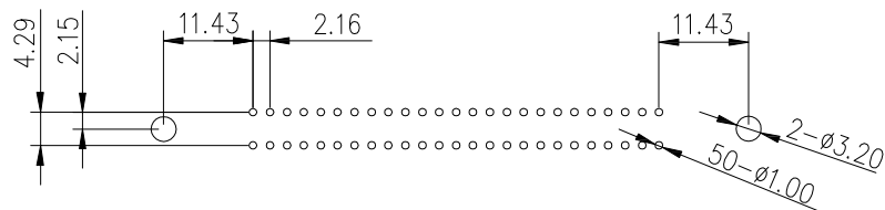
PCB layout
