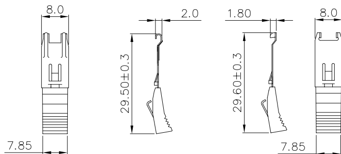
Flag hooks
