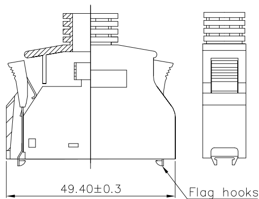
Flag hooks
