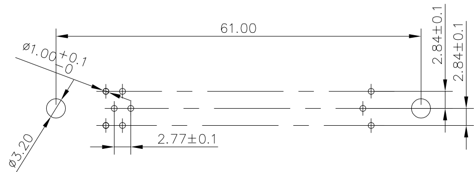
PCB layout
