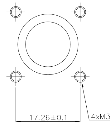
Mounting dimensions
