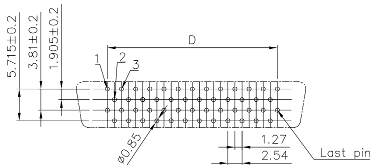
PCB layout A(26pin,50pin)
