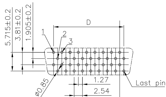
PCB layout A(20pin,36pin,40pin,68pin,100pin)
