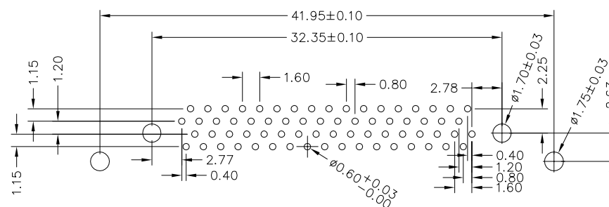
PCB layout
