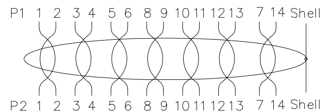
Pin assignment
