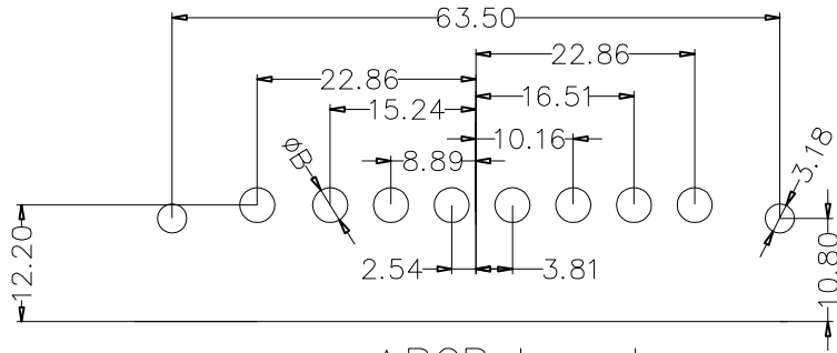
△PCB layout
