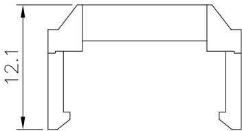
Strain Relief
