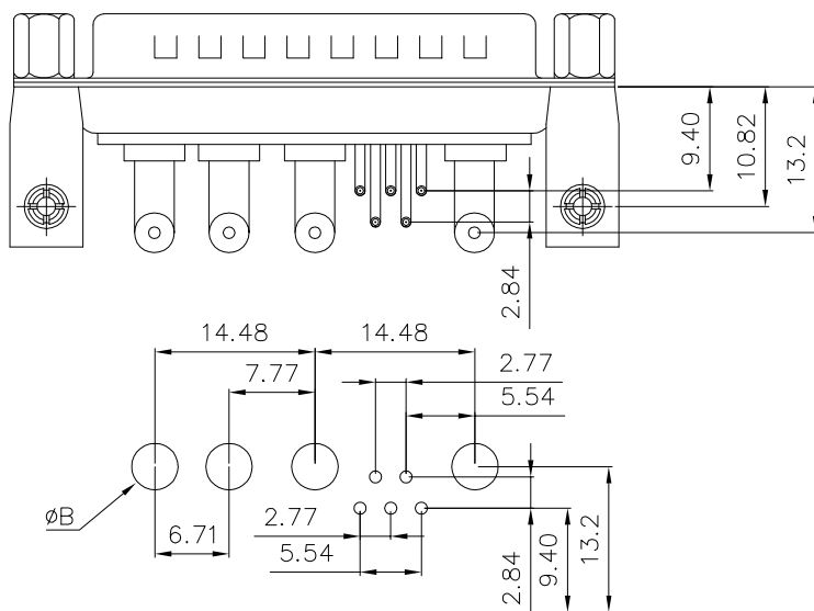
PCB LAYOUT
