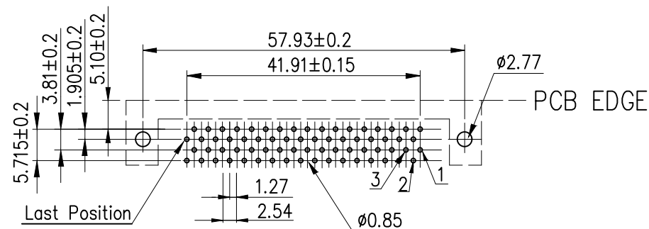
PCB layout
