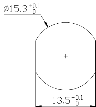
面板开板尺寸
