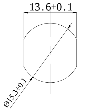
面板开板尺寸
