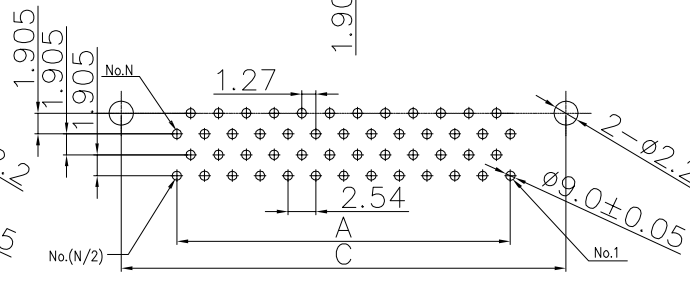
PCB Layout (30,50Pin)
