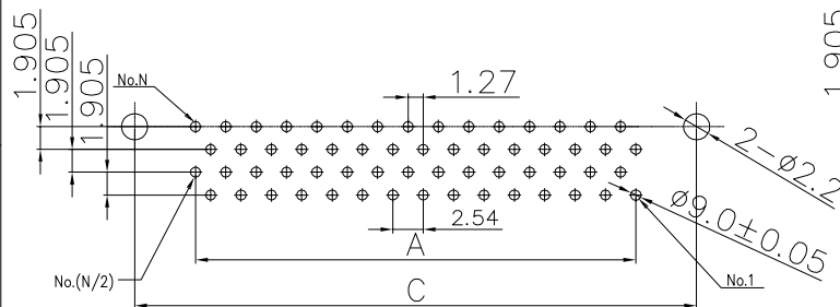
PCB Layout (40,60,80,100,120Pin)
