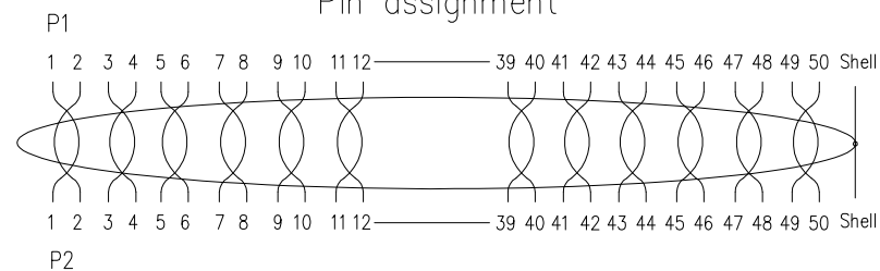
Pin assignment
