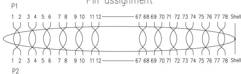
Pin assignment
