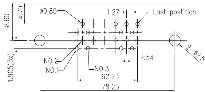
PCB layout
