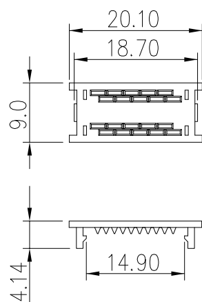
Termination Cover (1 Places)
