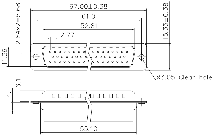
50 Positions
