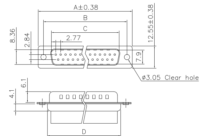
9,15,25,37 Positions
