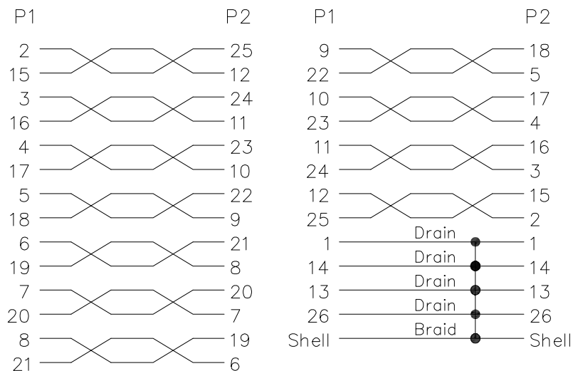
Wire assignment:
