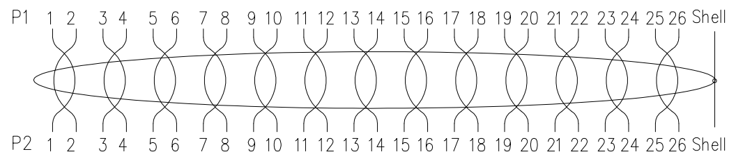
Pin assignment
