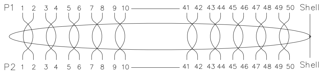
Pin assignment
