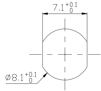
面板开板尺寸
