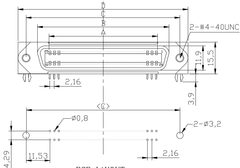
PCB LAYOUT
