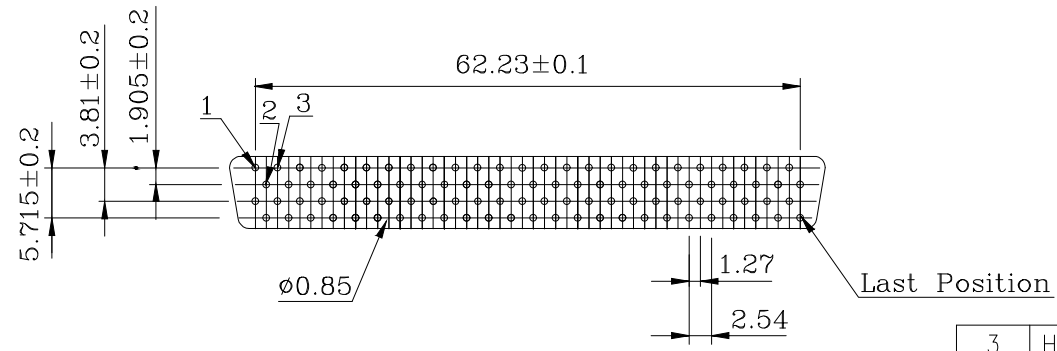
PCB Layout (B2)
