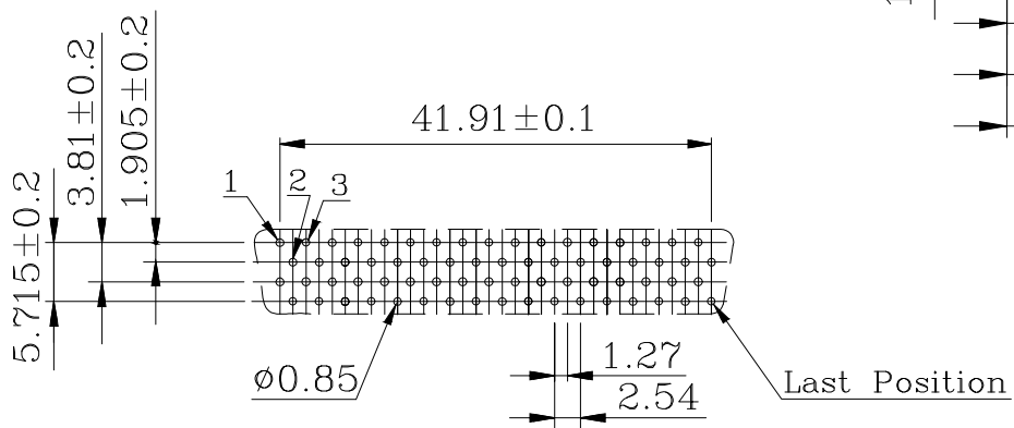
PCB Layout (B2)
