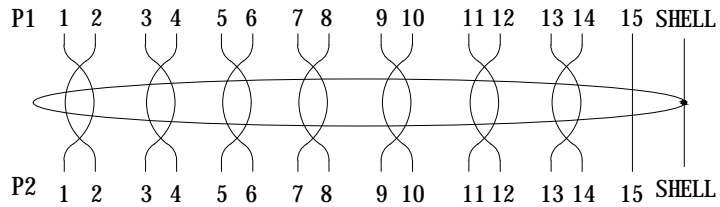
PIN ASSIGNMENT
