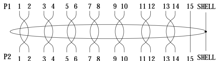
PIN ASSIGNMENT
