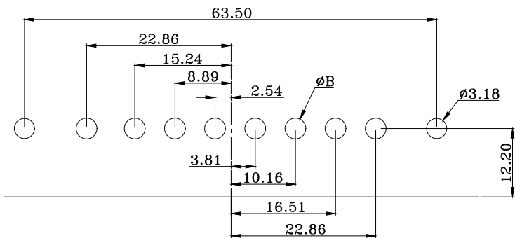
PCB LAYOUT
