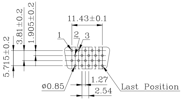
PCB Layout
