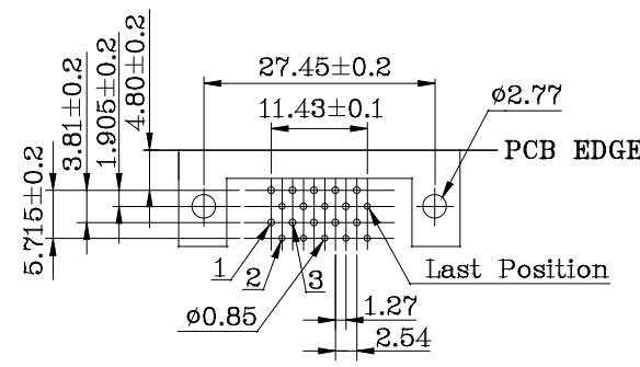
PCB Layout (B)
